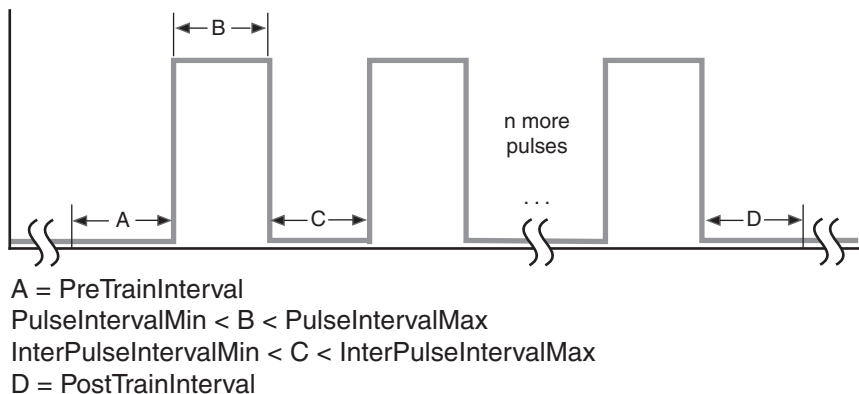
Figure 17. Pulse Train Timing, Receive
