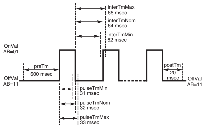
Figure 7. Example of T1 Loop Start Train Signal (0xC15CA032)
