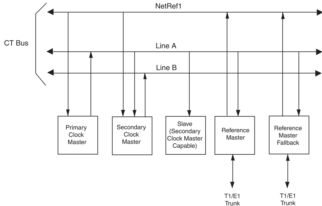
Figure 2. Clock Fallback
