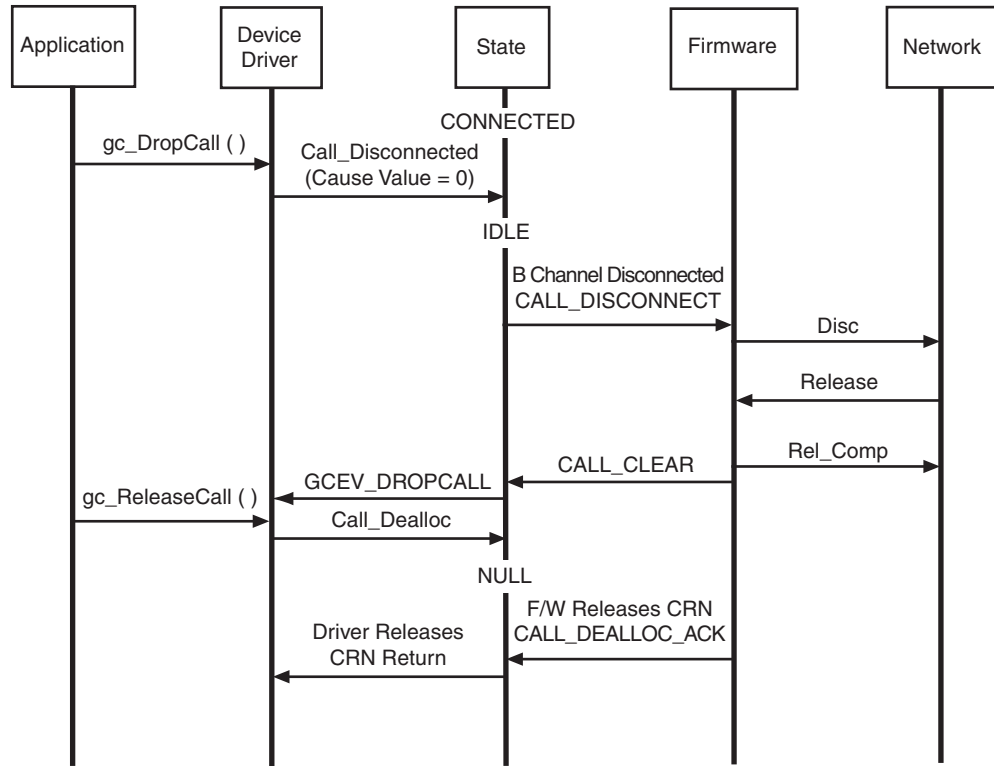
Figure 16. Application-Terminated Call (Asynchronous Mode)
