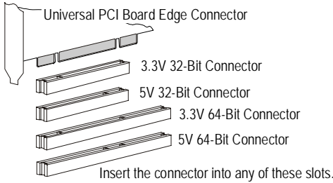
Figure 2. PCI Slots
