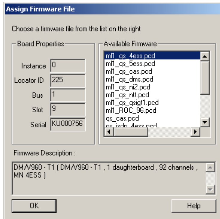
Figure 13. Assign Firmware File Dialog Box
