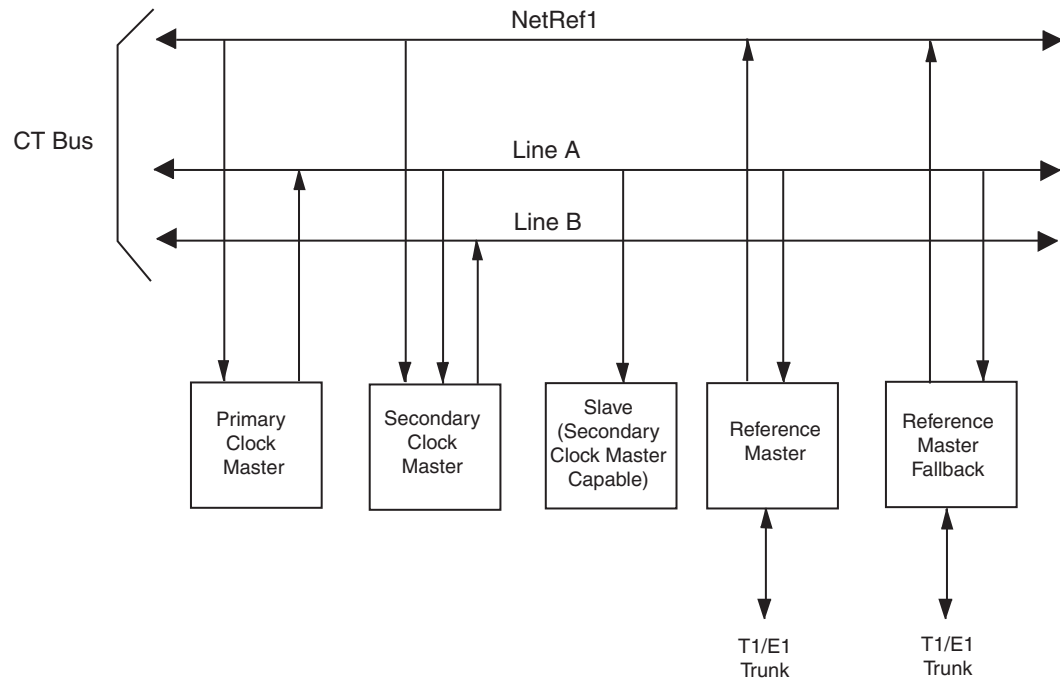
Figure 5. Clock Fallback
