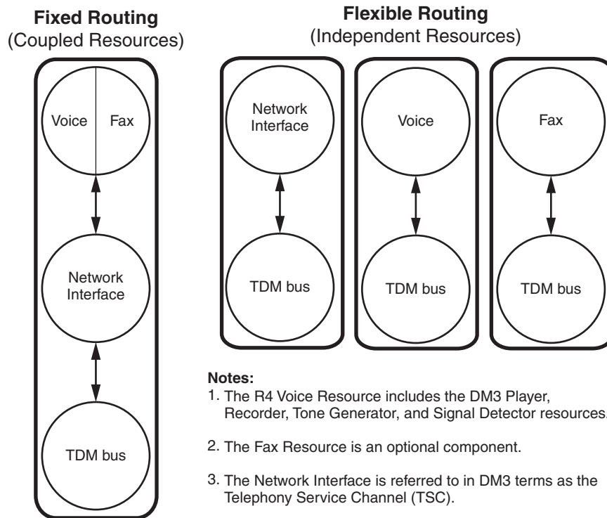
Figure 4. Cluster Configurations for Fixed and Flexible Routing
