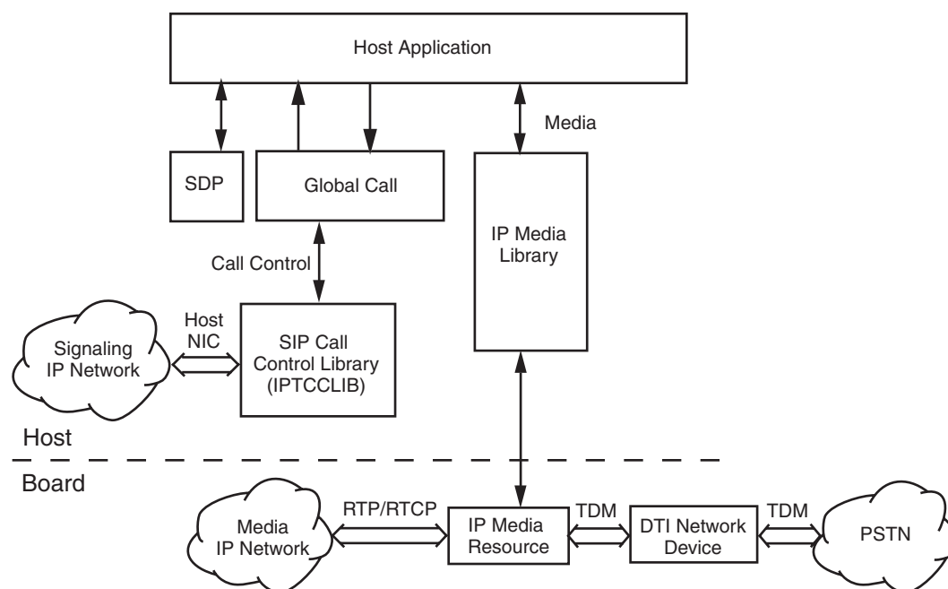
Figure 58. Global Call over IP Architecture for Third Party Call Control Mode
