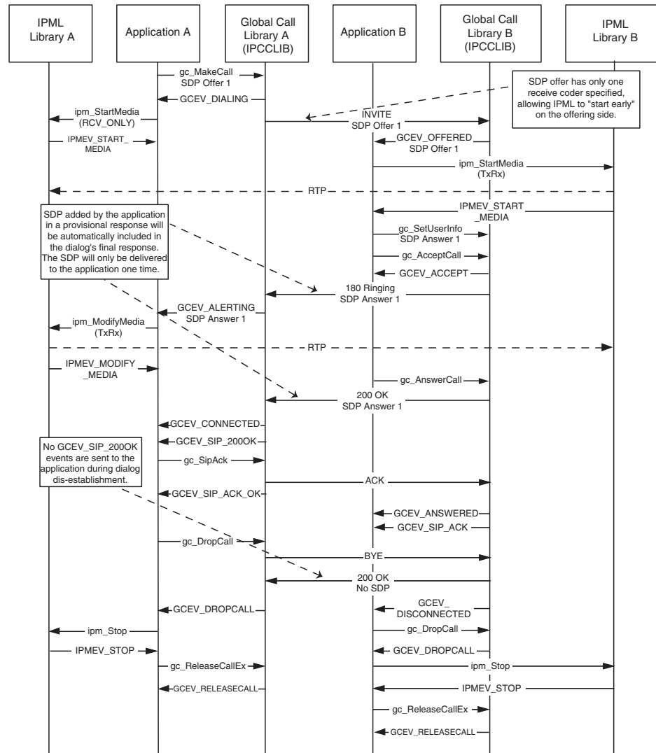
Figure 59. First Party Call Control Establishment in Third Party Call Control Mode
