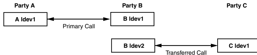
Figure 51. Global Call Devices for H.450.2 Blind Call Transfer or SIP Unattended Transfer
