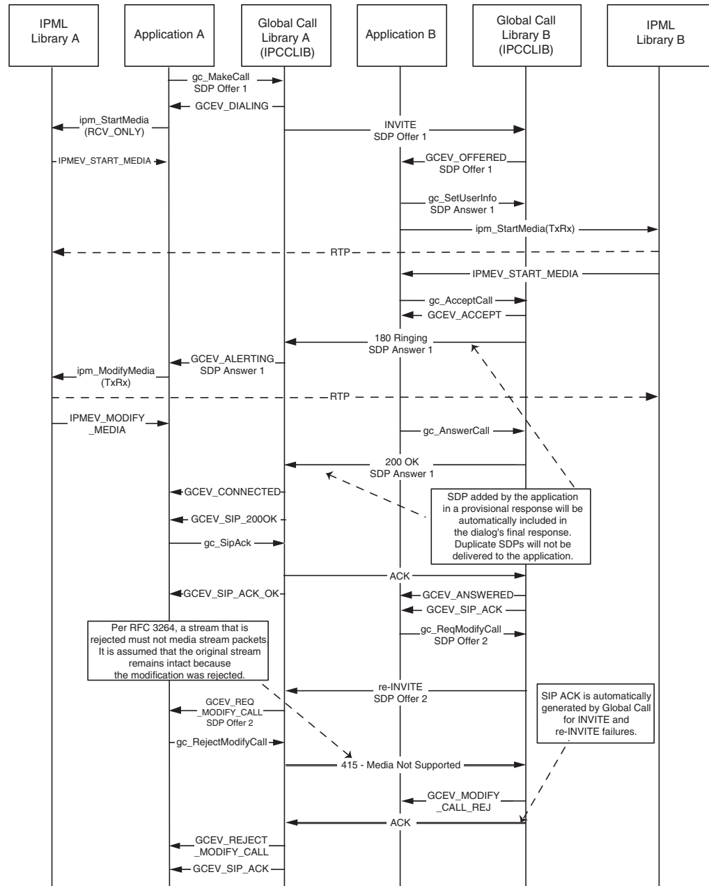
Figure 67. Unsuccessfully Modifying the Coder
