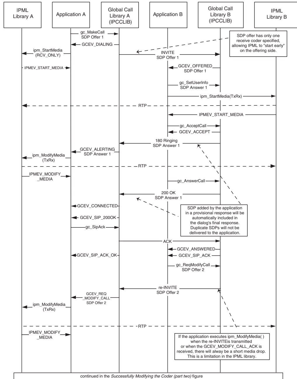
Figure 65. Successfully Modifying the Coder (part one)
