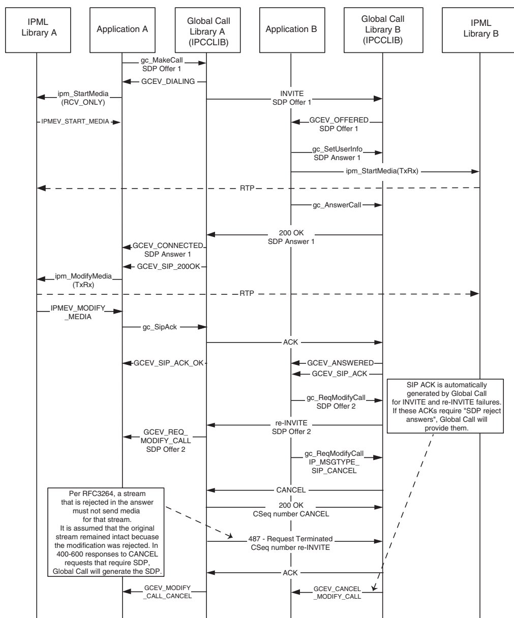
Figure 68. Cancelling a Coder Switch using re-INVITE
