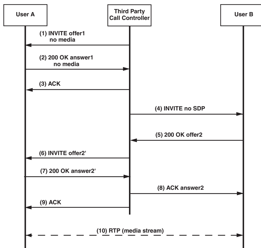
Figure 57. Third Party Call Control Setup using re-INVITE
