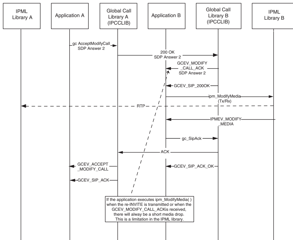
Figure 66. Successfully Modifying the Coder (part two)
