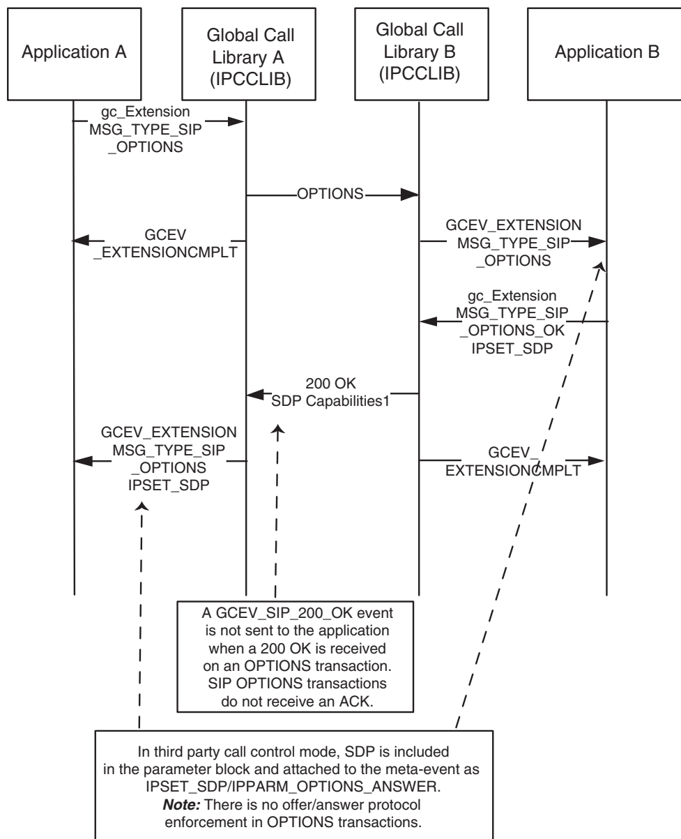
Figure 70. OPTIONS Request without a MIME Body
