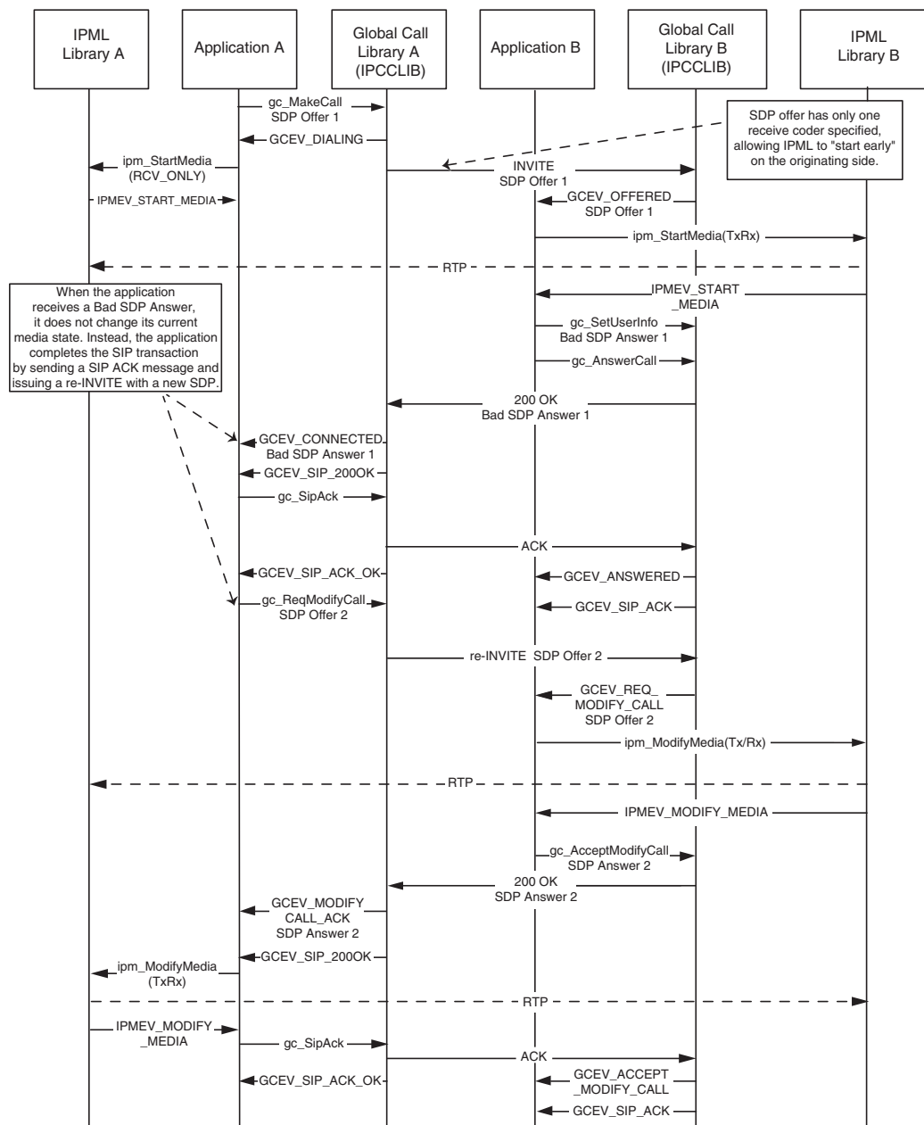
Figure 69. Receiving an Invalid Answer SDP
