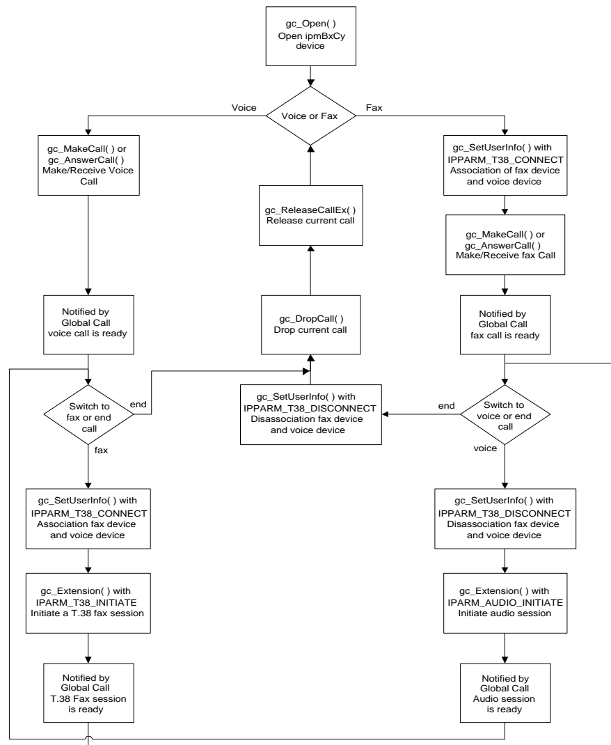
Figure 54. T.38 Fax Server Support in Manual Mode
