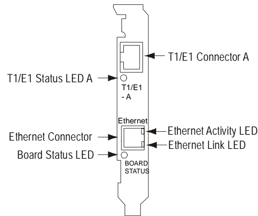
Figure 6 Front View of Mounting Bracket
