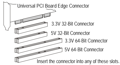
Figure 5 PCI Slots
