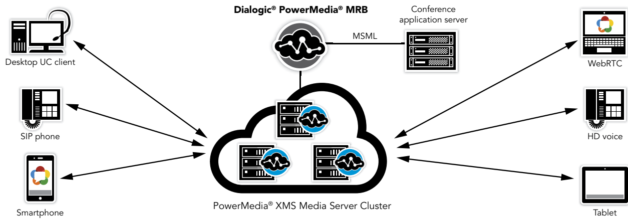
Figure 1 - High-scale audio conference example using a variety of SIP and WebRTC endpoints
